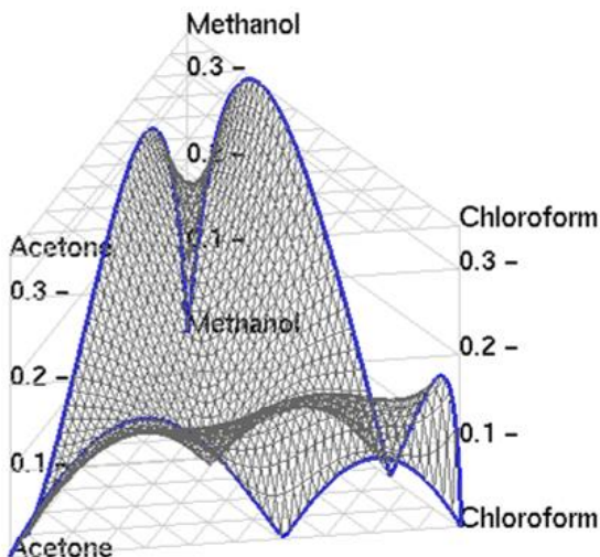
Figure 9: Deviation diagram.
